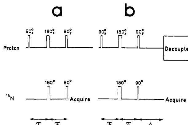
Figure 1. Pulse sequences used for obtaining 1NEPT enhanced spectra (a) without proton decoupling and (b) with proton decoupling. For the spectra of Figure 2a \tau was 2.5 ms and \Delta 5 ms.
